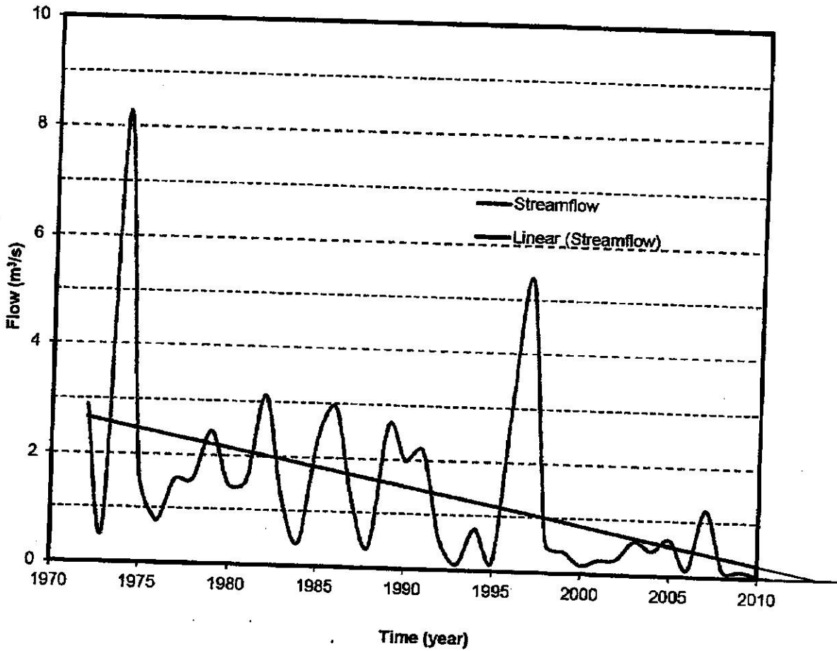
Figure 3.32 Trend on Mean Annual Flow of the Sturgeon River near Villeneuve
